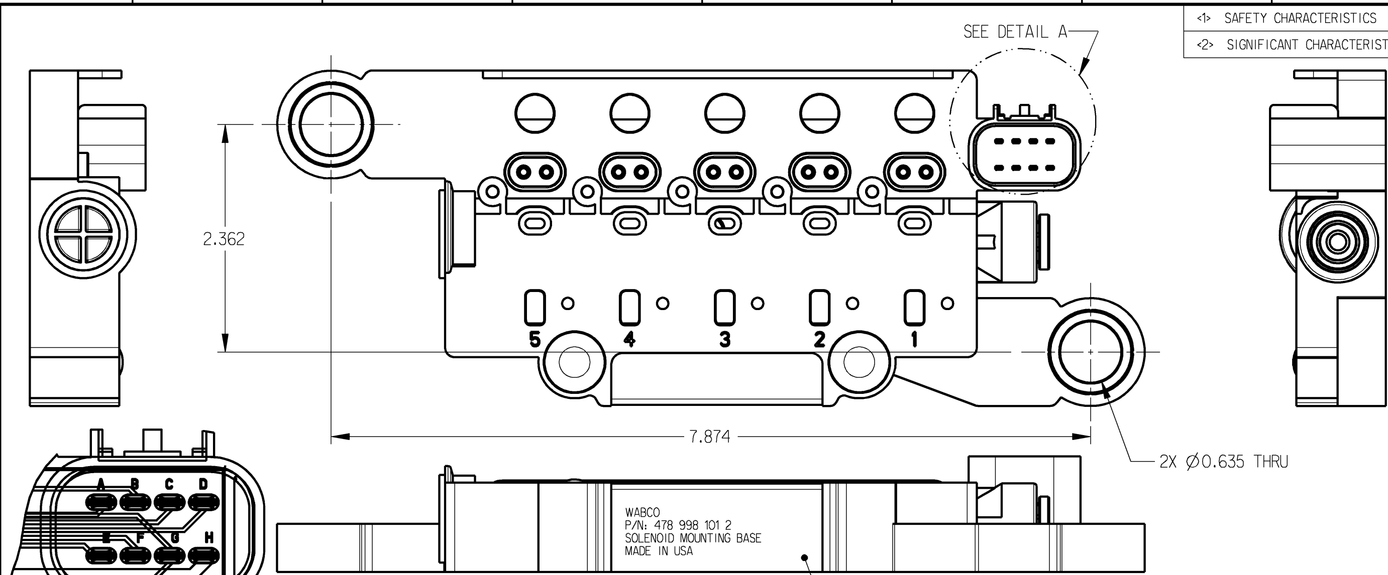
DETAIL "A" SCALE 2.0 PIN DESIGNATION
