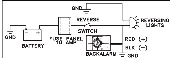
CONNECTION WITH FUSED REVERSE LIGHT CIRCUIT
