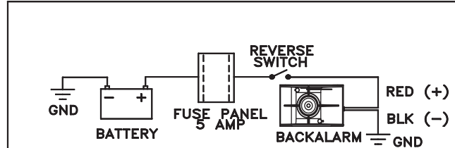
CONNECTION WITH SWITCH
